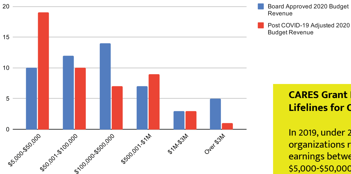
Change in Estimated Budgeted Revenue for Organizations
